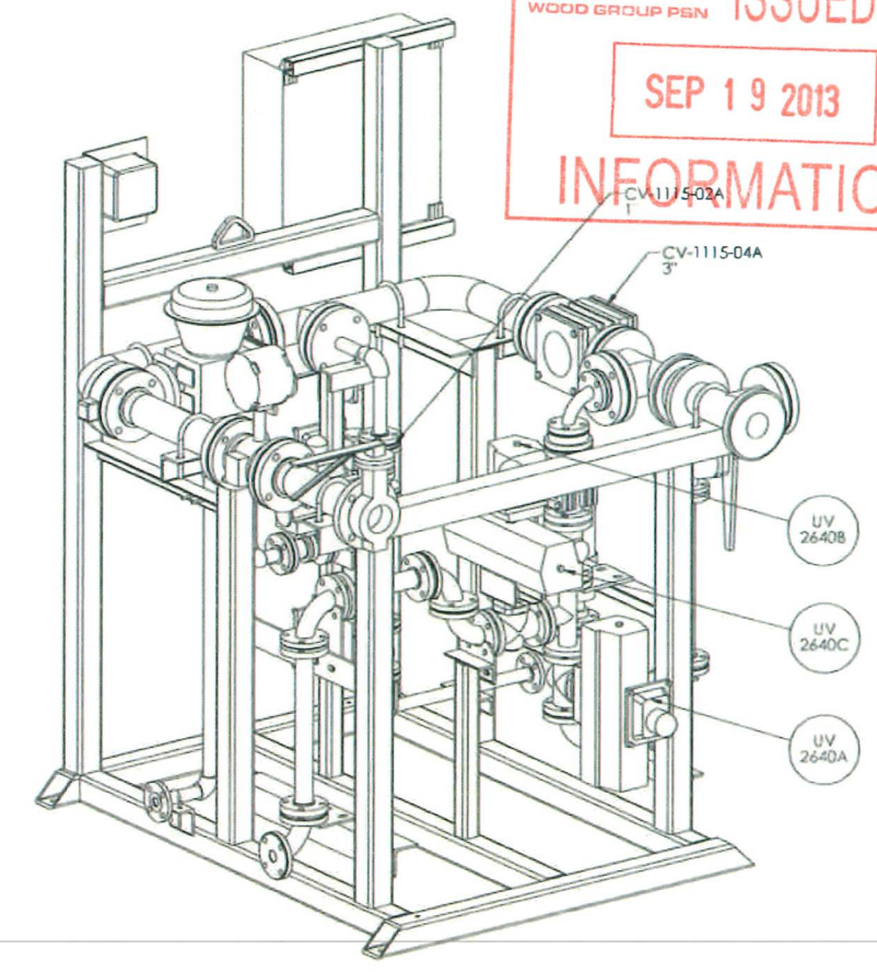
REAR ISO VIEW
