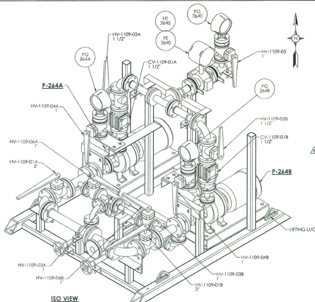
ISO VIEW
