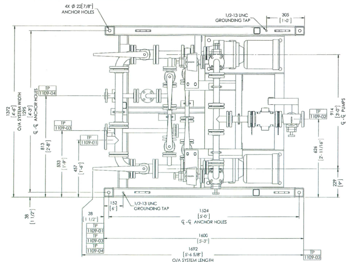
PLAN VIEW
